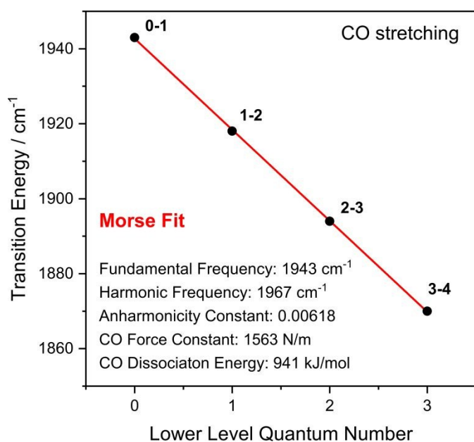
Figure 4: Transition energies observed for the CO stretch vibration of oxidized ReRH in the Ni_5^+ S state. Indicated bond properties were determined by fitting a function representing energy level separations of a Morse potential (red line) to the experimental data (black dots). Transitions between vibrational eigenstates |m\rangle and |n\rangle are labelled as m-n . For details, see SI2.
