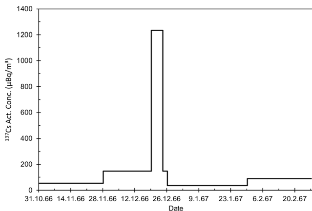
Fig. 6 The activity concentration of 137 Cs (µBq/m 3 ) in weekly air filters from Rovaniemi in 31.10.1966–28.2.1967, measured before combining the filters for pooled samples
