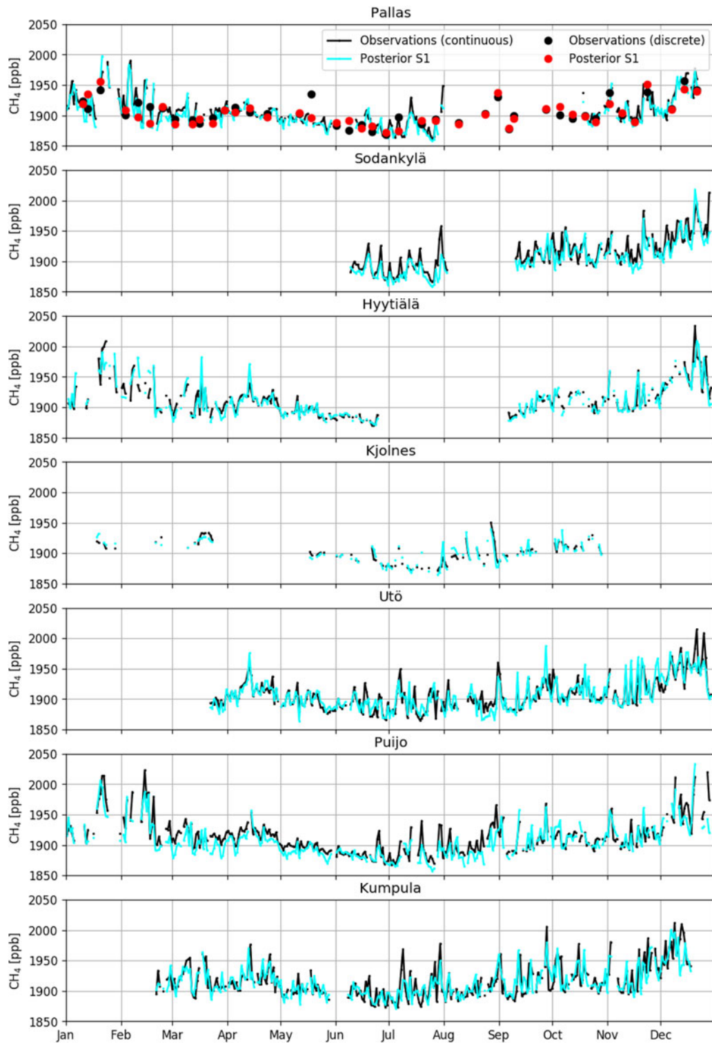
Fig. 2. Observed and simulated atmospheric CH 4 at sites in Finland and surrounding regions for 2012, except for Kjølnes which shows data from 2014. For continuous observations, the daily averaged values are shown. For complete time series for all inversions, see Supplementary Material .
