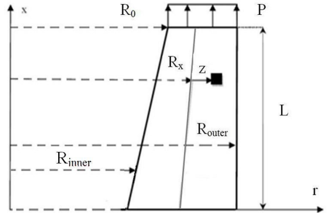
Fig. 1. Longitudinal section of shell subjected to axial stress at x=L
