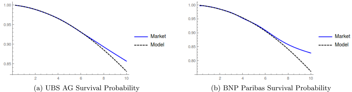
Figure 3.2: Dependence of the error on the maturity
