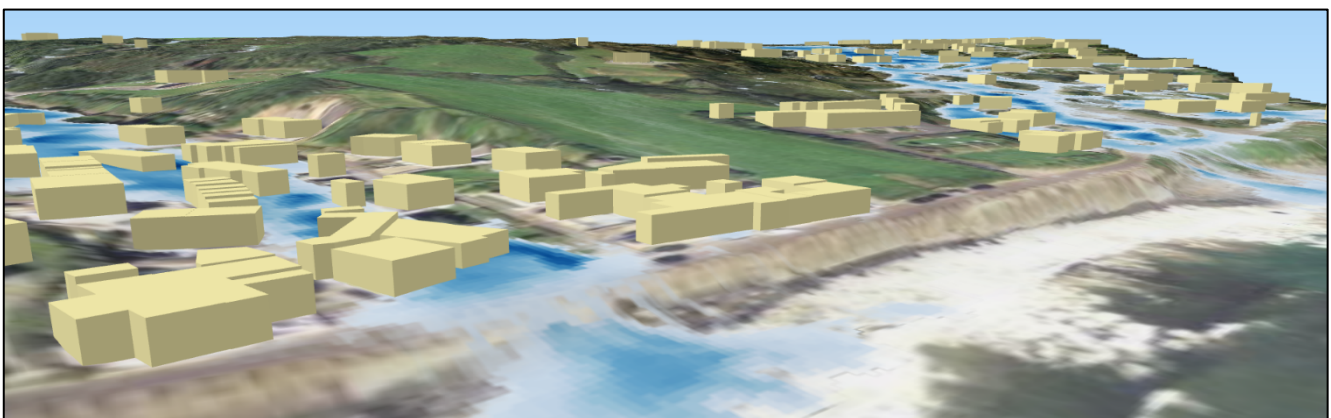
Figure 21. Example of Exeter hydrodynamic model of Coverack flood (Source: Albert Chen, the University of Exeter from the FFIR Research summaries)
