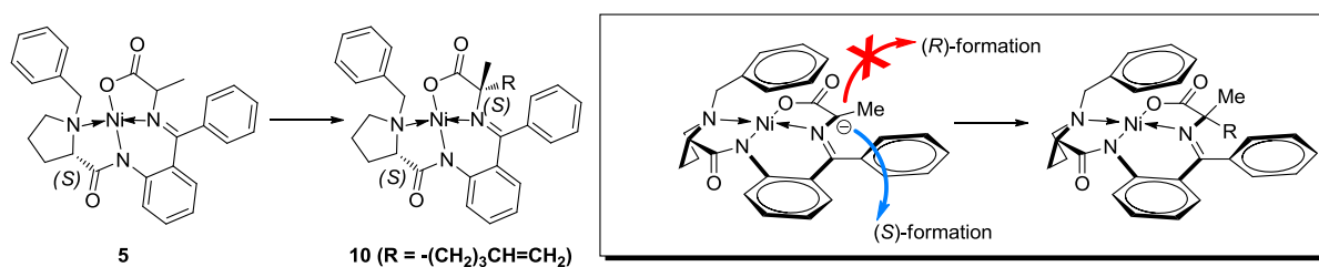
Figure 2. Mnemonic developed to rationalise stereoselective alkylation.
