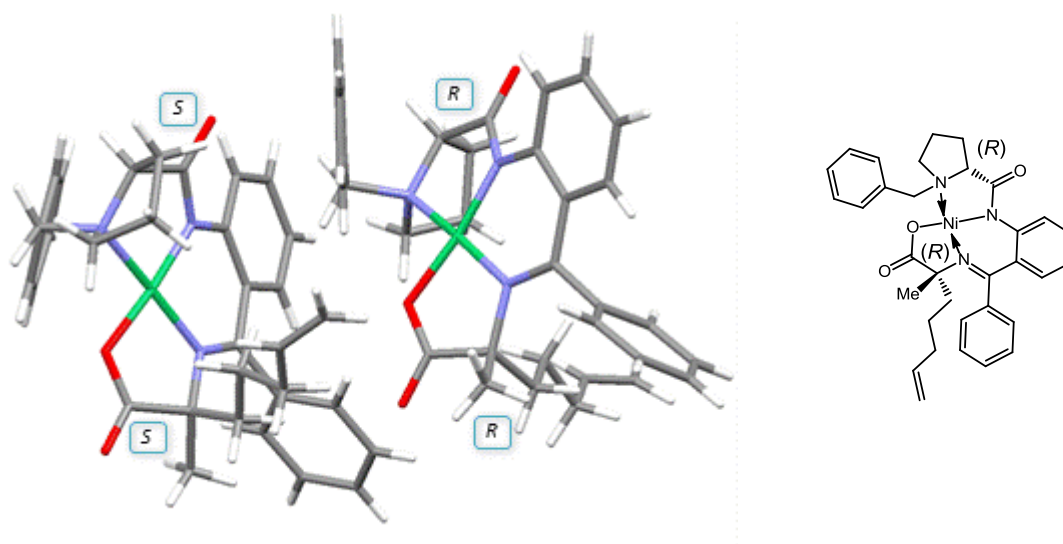
Figure 3. X-ray diffraction derived structure of BPB-complex 10 showing presence of opposite enantiomer.
