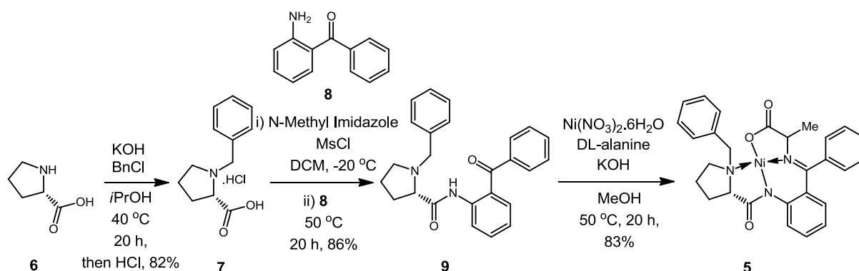
Scheme 1. Access to the BPB auxiliary.
