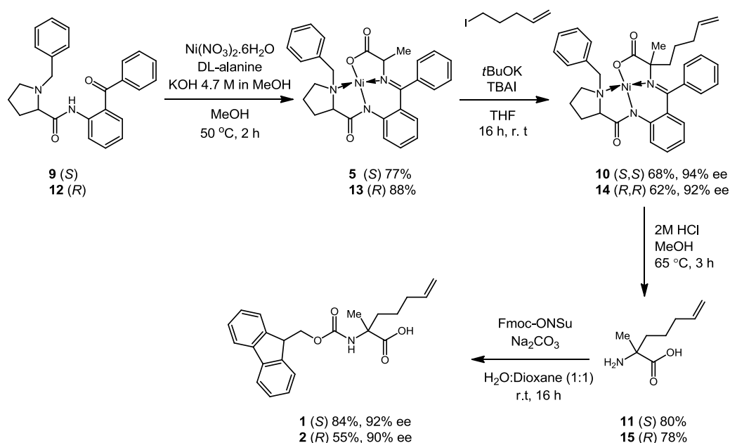
Scheme 3. Modified route to 1 and application to synthesis of 2 .
