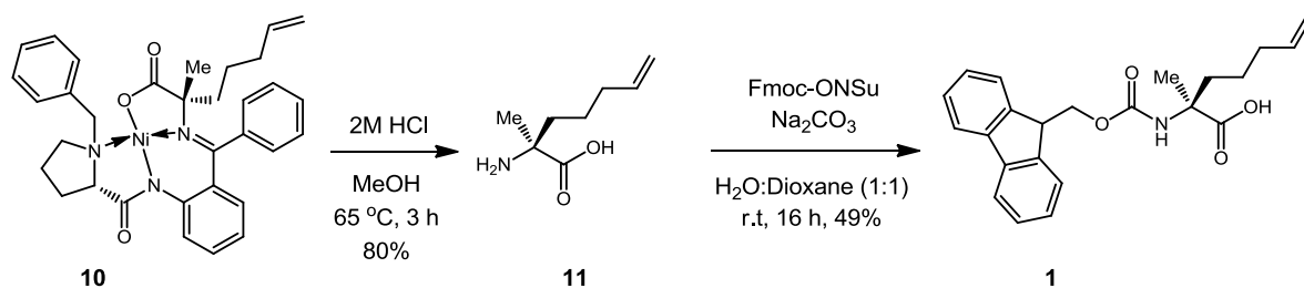
Scheme 2. Hydrolysis and Fmoc protection of final alkenyl amino acid.
