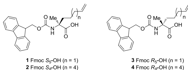
Figure 1. Verdine amino acids used for construction of peptide staples.
