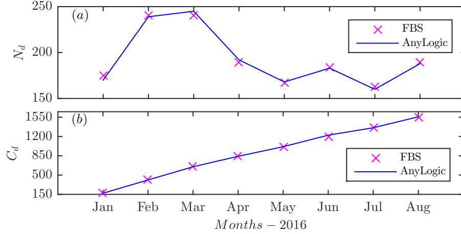
Figure 8: Simulation results against the FBS case study for the total number of dispatches (a) in each month N_d and (b) the cumulative monthly sum of the number of dispatches C_d between January and August 2016.
