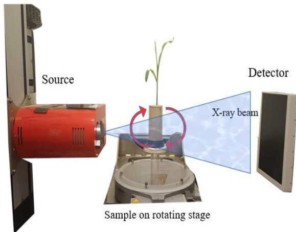
Fig.2. X-ray micro tomography set-up used to image the root-soil systems in a cylindrical specimen. The sample is placed on a rotation table and the distance between the x-ray source, the sample and the detector was fixed throughout the whole observation.
