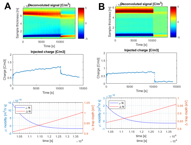
Fig. 3- Apparent charge mobility and trap depth at 60°C for non-filled (A) and filled (B) materials. Results from thick cast film samples.
