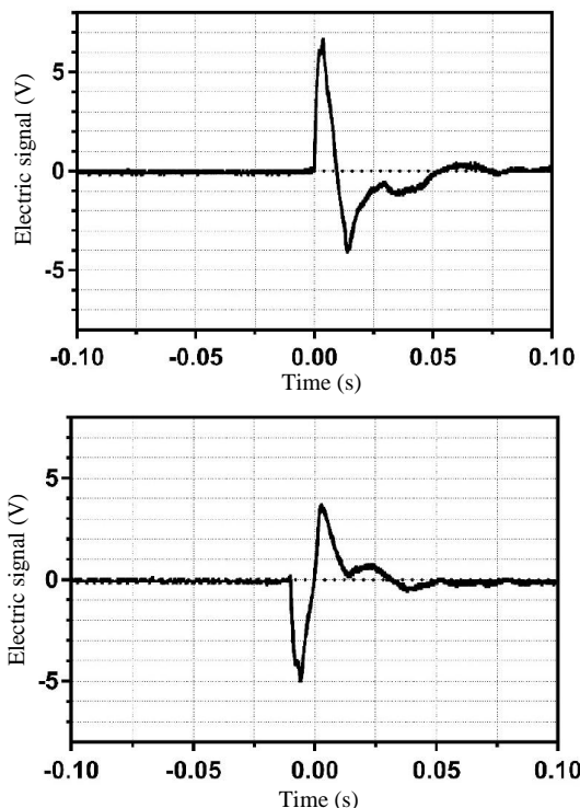
Fig. 6. Electric response to mechanical impact of 100g mass falling from 3 cm height. Sample in direct (A) and inverted (B) position.
