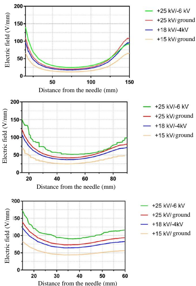
Fig. 2. FEM results. Interelectrode electric field (max value) as a function of the position from the needle for different voltage applied to the needle (+) and the collector (- or ground). Needle-collector distance of 150 mm (A), 90 mm (B) and 60 mm (C).
