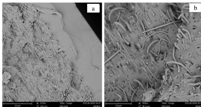
Fig. 5. SEM pictures of PDMS + nanofibrous mat sample. Magnifications: 2500X (A), 7000X (B)
