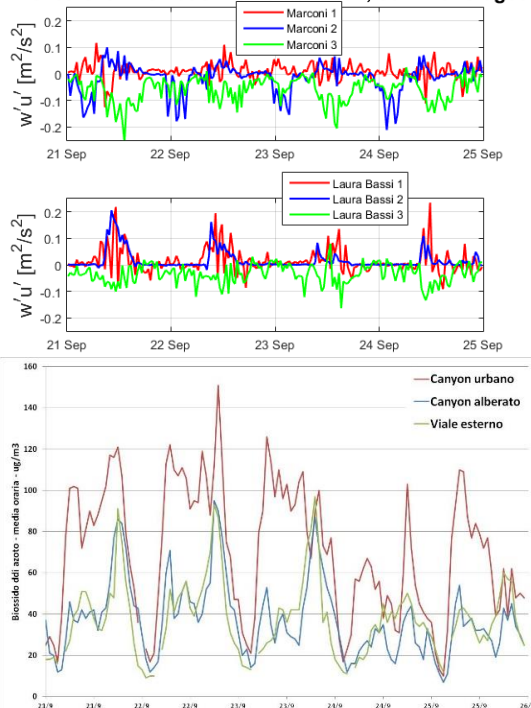
Turbulent kinematic momentum flux, 30min averaged
