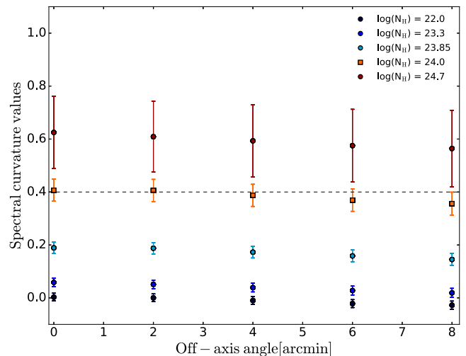
Figure 4. Spectral curvature values as function of the off-axis position for simulated AGNs with different column densities N_{\text{H}} , redshift z = 2 and with intrinsic luminosity of 5 \times 10^{44} \text{ erg s}^{-1} . The deviations in the SC values due to the off-axis position are small compared to the error bars.
