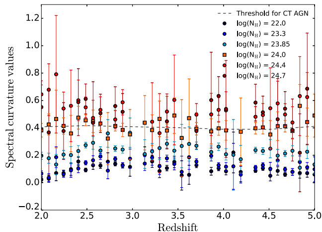
Figure 2. Normalized SC values of simulated sources versus the redshift. The SC method selects sources with column densities above 10^{24} \text{ cm}^{-2} as CT AGNs. Thus, the SC method successfully distinguishes CT sources from merely obscured AGNs.
