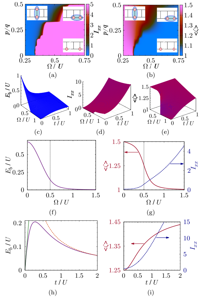
FIG. 2. (Color online) M = 2 . (a) and (b): “Phase diagram” of two particles showing dependence of (a) I_{xx} and (b) \langle \zeta \rangle on flux p/q and \Omega/U for t/U = 0.1 . The insets show the type of bound state stabilized. (c)–(e), p/q = \frac{1}{2} : E_b , I_{xx} , and \langle \zeta \rangle are respectively shown in (c)–(e). (f) shows the dependence of E_b on \Omega/U for t/U = 0.1 , while (g) shows I_{xx} and \langle \zeta \rangle for the same case. The vertical black dotted lines show \Omega = \Omega_c . The dependence of E_b in (h) and I_{xx}, \langle \zeta \rangle in (i) on t/U at \Omega = \Omega_c = U/2 are shown. The dashed lines in (h) are results of analytical considerations at small and large t/U .
