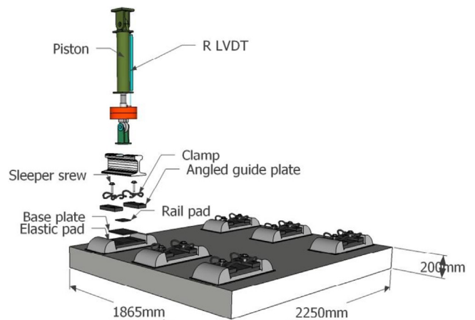
Fig. 5. Tack system and loading configuration.
