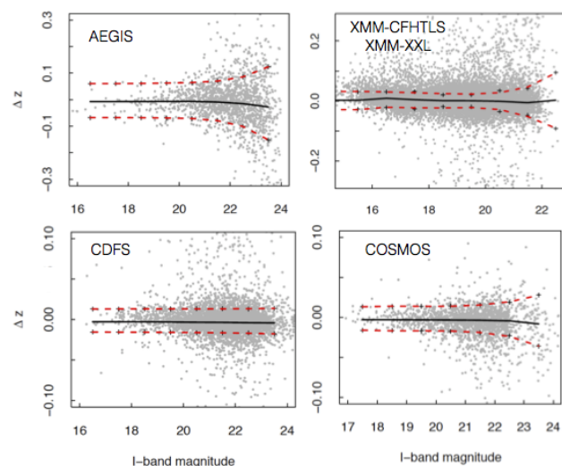
Fig. 3. Same as Figure 2 but for the AEGIS, COSMOS, CDFS, XMM-CFHTLS, and XMM-XXL fields.
