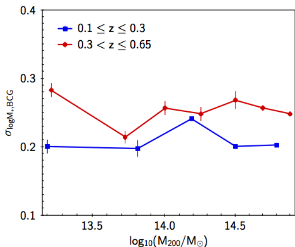
Fig. 6. Scatter in the stellar mass of BCGs at a given halo mass in low and high redshift bins. The scatter is the quadratic sum of intrinsic scatter and measurement scatter of stellar masses.
