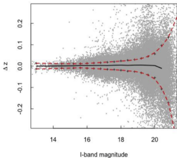
Fig. 2. Shown is the relation (Photometric redshifts - Spectroscopic redshifts) / (1 + Spectroscopic redshifts) ( \Delta z ) vs. i -band cModel magnitude for a sample of galaxies with both spectroscopic and photometric redshifts in SDSS DR14 (gray dots). The black pluses and black solid line show the dispersion and peak of the Gaussian fitted in each i -band magnitude bin, respectively. There are in total 17 bins. The red dashed lines indicate the model fitted to the dispersions.
