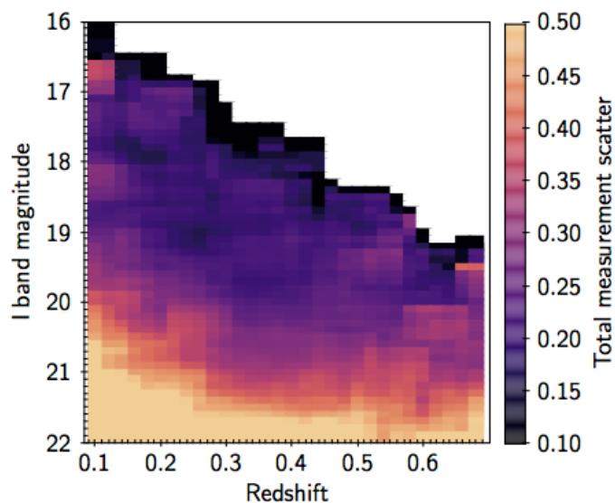
Fig. 7. Total measurement scatter in estimating stellar mass in redshift-magnitude space.
