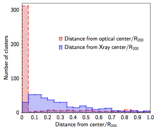
Fig. 4. Distance of the BCGs from the optical and X-ray centers normalized by R_{200} . Of the BCGs, 79% reside in \sim 0.05 \times r_{200} from optical center, and 92% and 84% of BCGs reside in 0.5 \times R_{200} from optical center and X-ray center, respectively.
