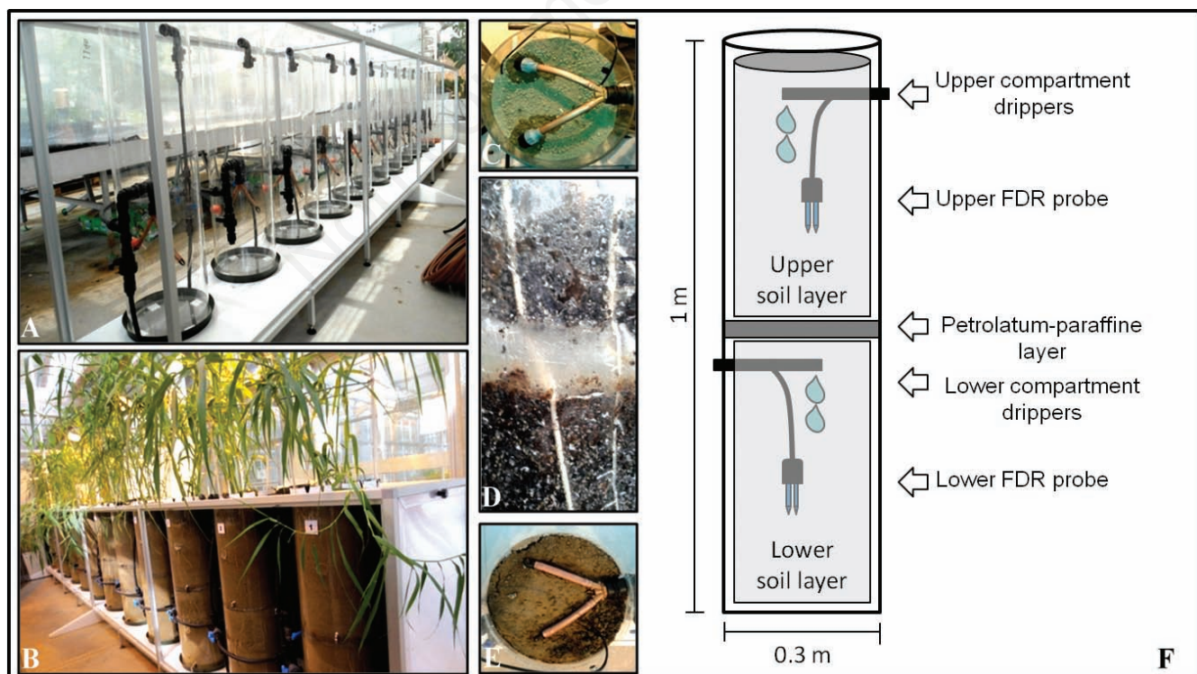
Figure 1. System set up: A) transparent cylinders (rhizotrons); B) system open for visual root determinations; C, E) sub irrigation (drippers); D) roots passing through the petrolatum/paraffin film; F) system outline.
