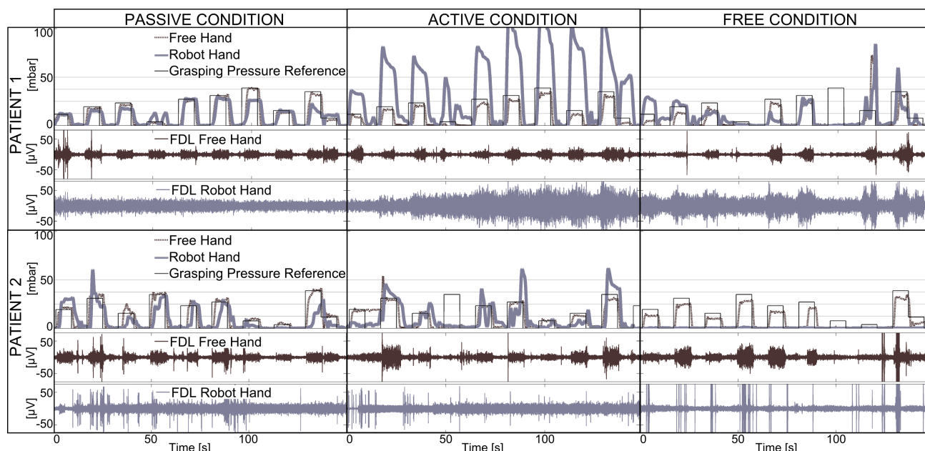
Fig. 15: Data acquired during the experimental session with stroke patients. Graphs are referred to the Active and Passive conditions (columns) and patients (rows), showing three representative bilateral grasping sequences
