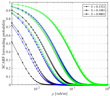
Fig. 8: SCARF forwarding probability for a vehicle within the source vehicle's transmission range z [m], versus the vehicular density \rho [veh/m] and for selected values of the social degree and of the shape factor, i.e. , c = [1, 2, 5] for black , blue and green lines , respectively.
