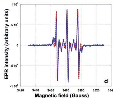
Fig. 4 EPR spectra of PDTSTzTz not wetted by DMPO solution, and irradiated with the solar simulator (a) under argon and; (b) in the presence of air ( g = 2.0023 ). EPR spectra of PDTSTzTz wetted by DMPO solution and irradiated (c) under argon; (d) in presence of air. Parts (c) and (d) show the experimental spectra (solid blue line) together with their simulations (dotted red line).
