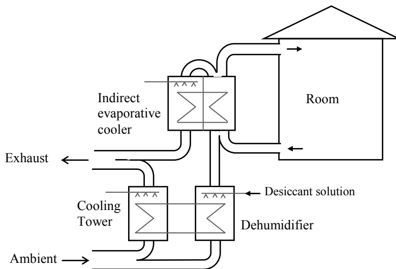
33 34 Fig. 3: Schematic of liquid desiccant cooling configuration with indirect evaporative cooling of 35 external air mixed with recirculating internal air [33] 36
