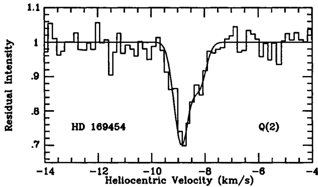
Figure 2. A two-component fit to the Q(2) line towards HD 169454 with the line profile parameters given in Table 4.
