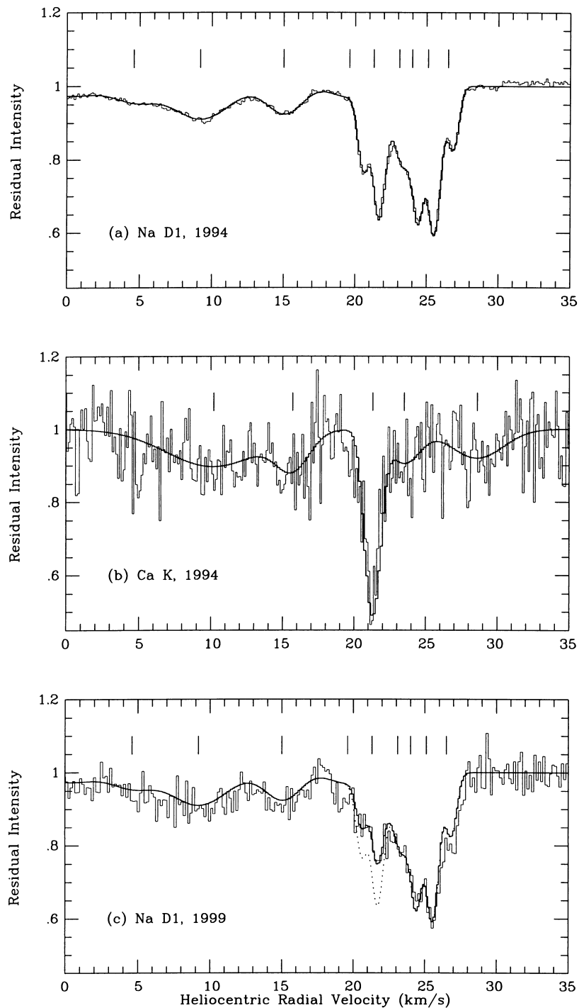
Figure 1. Theoretical line profiles are shown plotted over spectra observed toward \delta Ori A in the (a) Na I and (b) Ca II regions, both obtained in 1994, and (c) Na I region, obtained in 1999, with the fit to the 1994 data (dotted line) superposed. The tick-marks indicate the velocities of the individual model components listed in Table 1.
