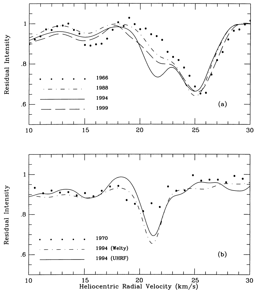
Figure 2. Comparison of (a) Na I and (b) Ca II observations towards \delta Ori A on the dates indicated (cf. Table 2). All the spectra have been reduced to a common, effective, resolving power of R = 2 \times 10^5 .
