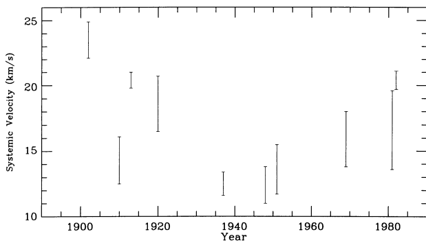
Figure 3. Systemic velocity measurements made of \delta Ori A, taken from table II of Harvey et al. (1987).
