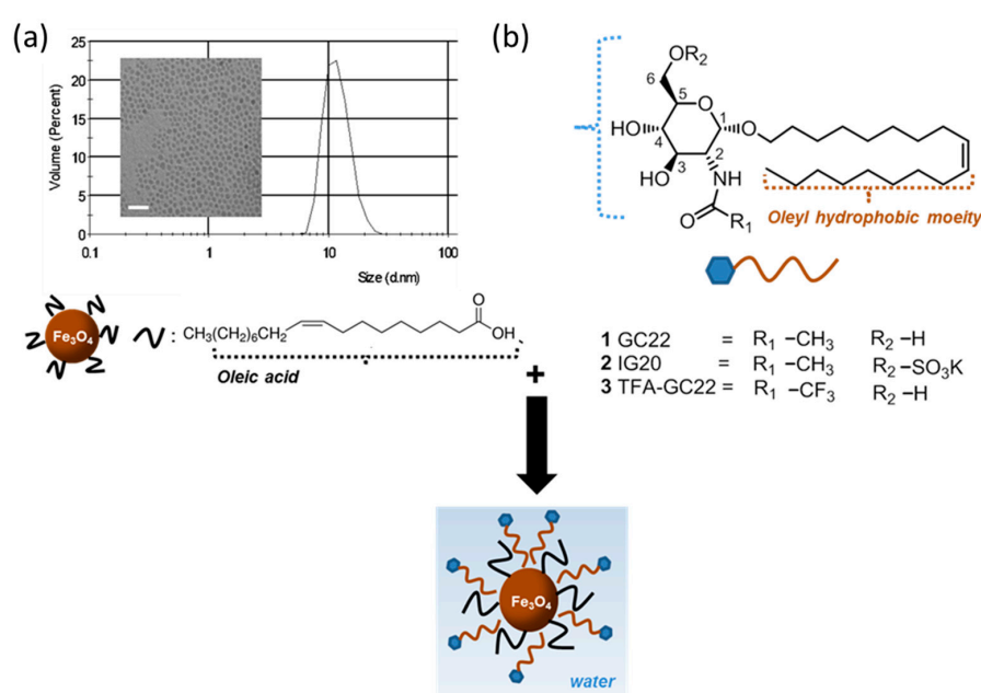
Figure 1. Scheme of the synthesis of the glycosides-coated IONP micelles. (a) Hydrodynamic size and TEM image (scale bar: 25 nm) of OA-IONP; (b) Structure of the bioactive glycosides.
