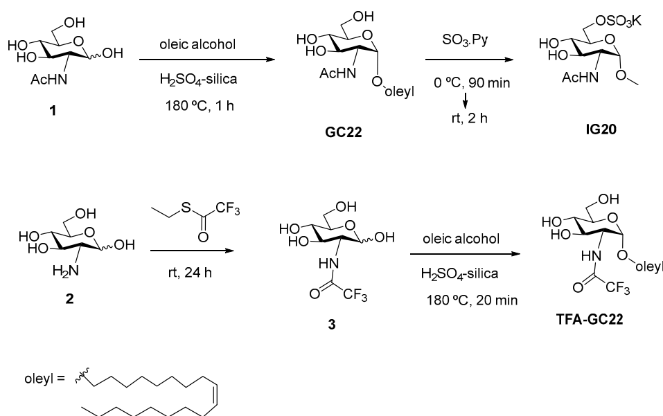
Figure 2. Synthesis of the glycosides GC22, IG20, TFA-GC22.
