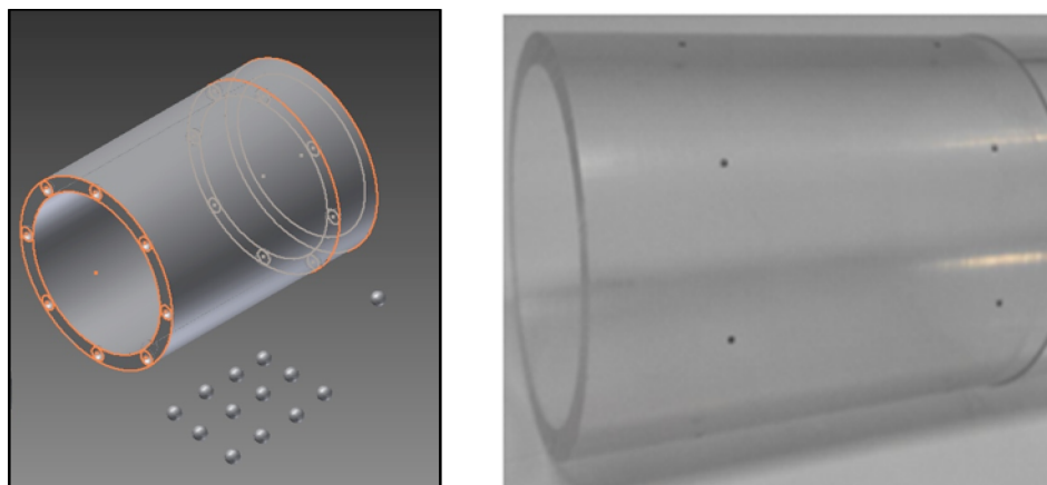
Fig 6. Design of the calibration phantom (left) and real phantom (right).
