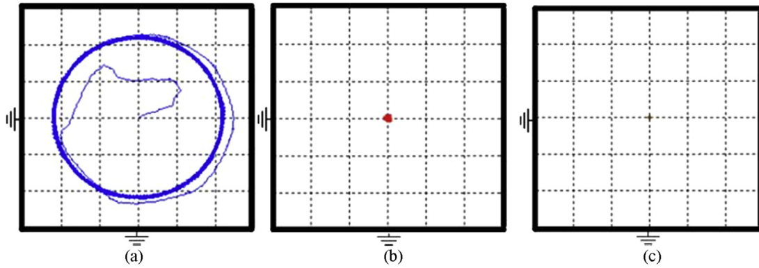
Fig. 7. Response trajectories in stationary reference frame current components. a. i_{s1} vs i_{s1} , b. i_{s5} vs i_{s5} , c. i_{s3} vs i_{s3} . [X–Y-axis scale: +/-10 A/div].
