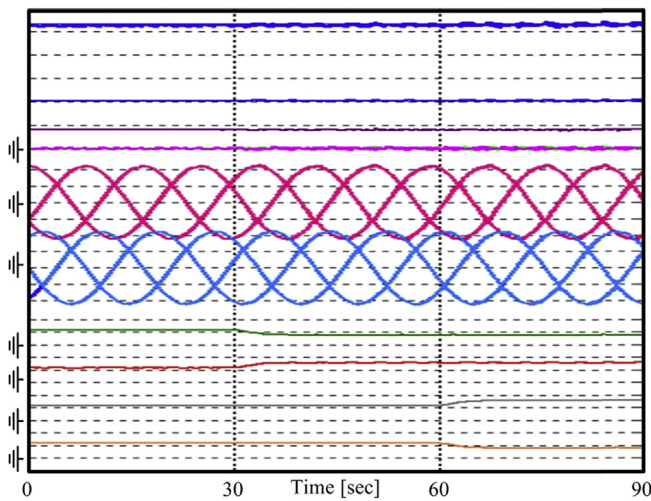
Fig. 6. Behavior of six-phase asymmetrical (quasi) open-end stator windings induction motor in first prediction when unbalanced voltage sharing between each couple of inverters ( VSI_H and VSI_L ) condition. Characteristic waveform in sequential order: a. Torque response with respect to step changes (blue-torque, red-step command). [Y-axis scale: 10 N m/div]. b. Torque producing current (first-space) component i_{1q} . [Y-axis scale: 10 A/div]. c. Flux producing current (first-space) component i_{1d} . [Y-axis scale: 10 A/div]. d. Leakage current (fifth-space) components i_{5q} , i_{5d} . [Y-axis scale: 10 A/div]. e. Three-phase current of first open-end stator windings. [Y-axis scale: 10 A/div]. f. Three-phase current of second open-end stator windings. [Y-axis scale: 10 A/div]. g. DC link current of inverter VSI_H^{(1)} . [Y-axis scale: 10 A/div]. h. DC link current of inverter VSI_L^{(1)} . [Y-axis scale: 10 A/div]. i. DC link current of inverter VSI_H^{(2)} . [Y-axis scale: 10 A/div]. j. DC link current of inverter VSI_L^{(2)} . [Y-axis scale: 10 A/div].
