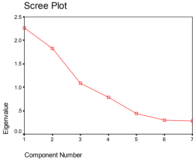
Figure 4.1 The scree plot representing the amount of variance explained by each variable. Note that the “breakage point is between 3 rd and 4 th points.
