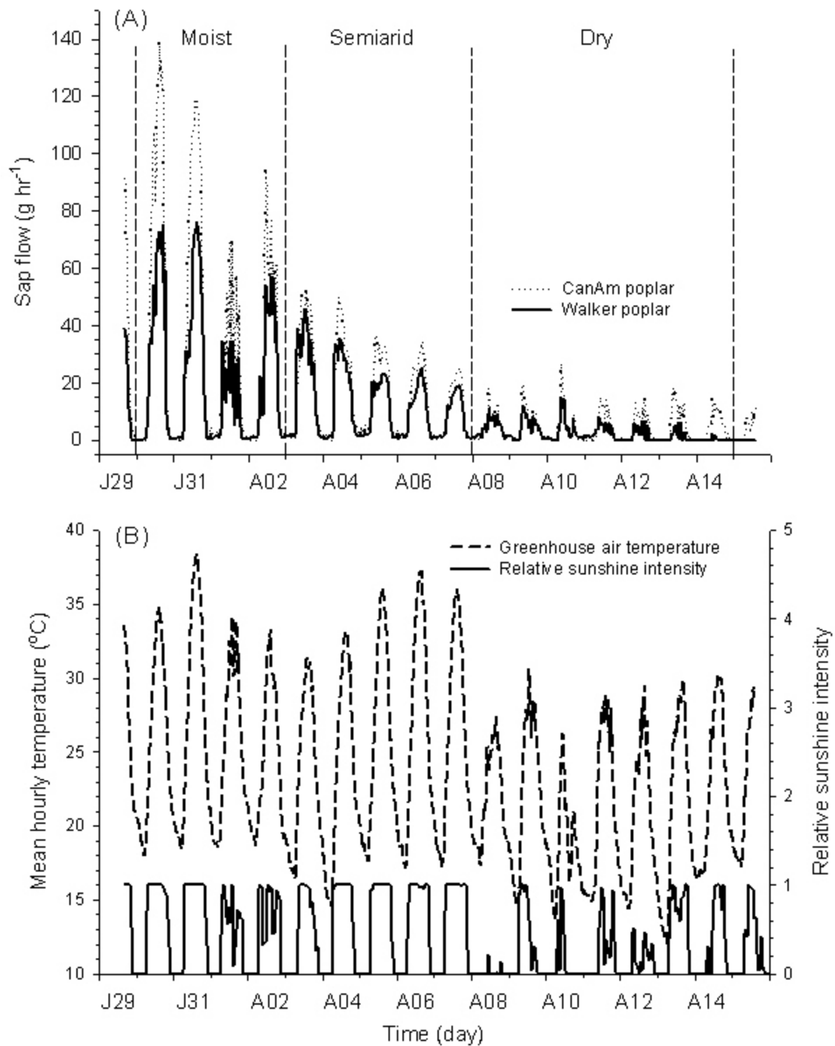
Figure 1. (A) Mean sap flow (g hr -1 ) adjusted for leaf area, as soil conditions progressed from moist to dry (July 29 th to August 15 th , 2005), as measured by Dynamax (Model SGA-10) heat flow gauges mounted near the base of CanAm and Walker poplars, and (B) diurnal mean hourly greenhouse air temperature and relative sunshine intensity fluctuations.
