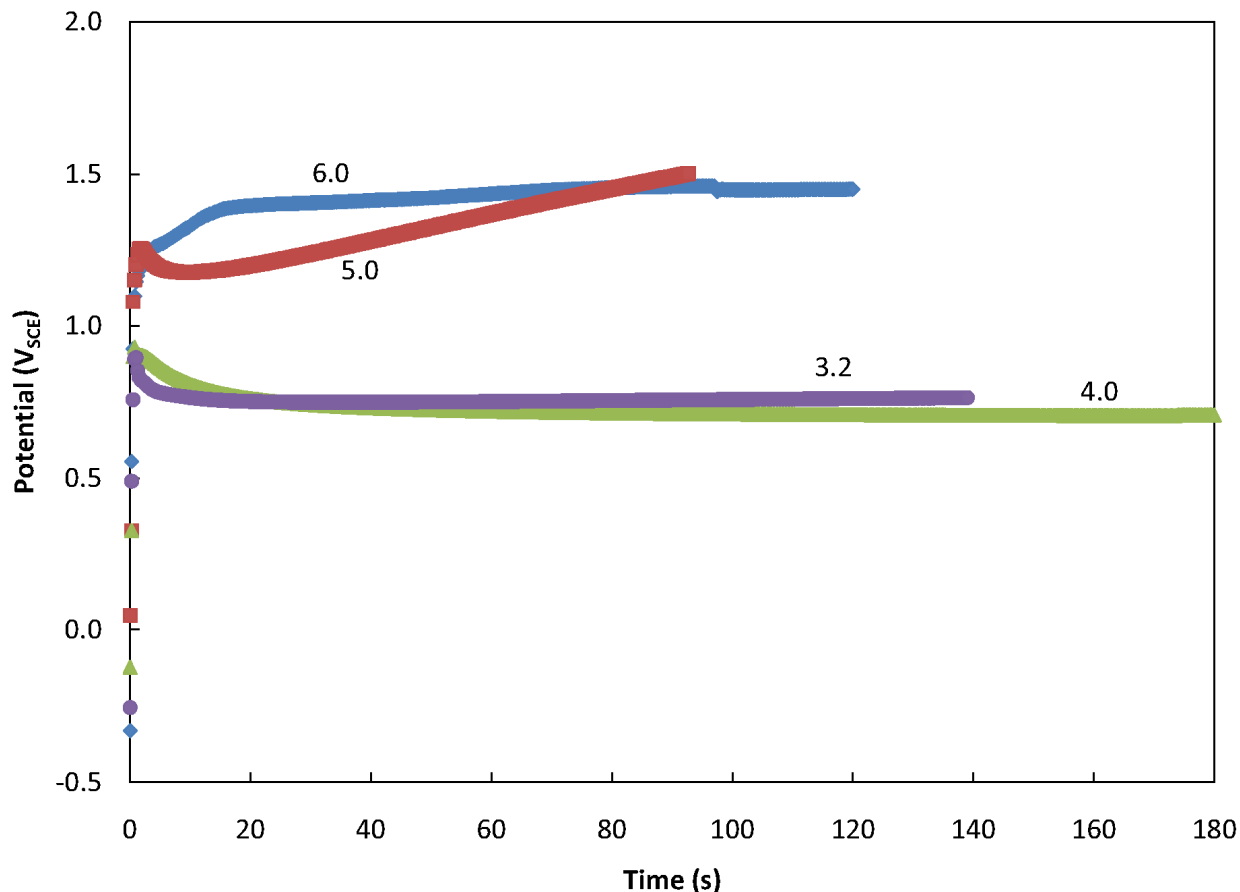
Figure 4.2. Chronopotentiometry plots for deposition of polypyrrole on stainless steel 304L from solutions of different pH (shown as labels). At values of 3.2 and 4.0, the polymer forms more easily and is more conductive than at higher values.
