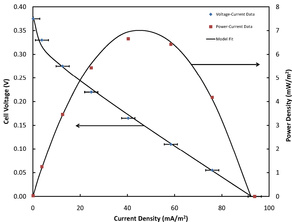
Figure 4.15. Polarization and power curves for bioanode/biocathode microbial fuel cell with soluble mediator graphite anode and immobilized mediator steel cathode along with fit to basic model. Error bars show the relative standard deviation of current measurements.
