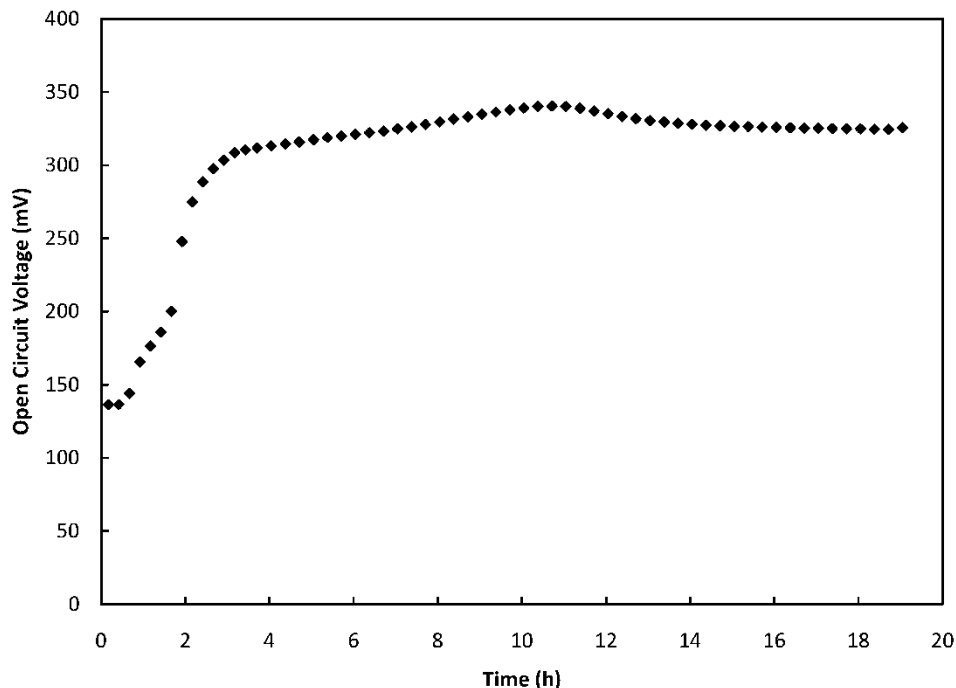
Figure 4.17. Evolution of the open circuit voltage of a biocathode/bioanode microbial fuel cell after inoculation with a starter culture of C. vulgaris in the cathode and a dry culture of S. cerevisiae in the anode.
