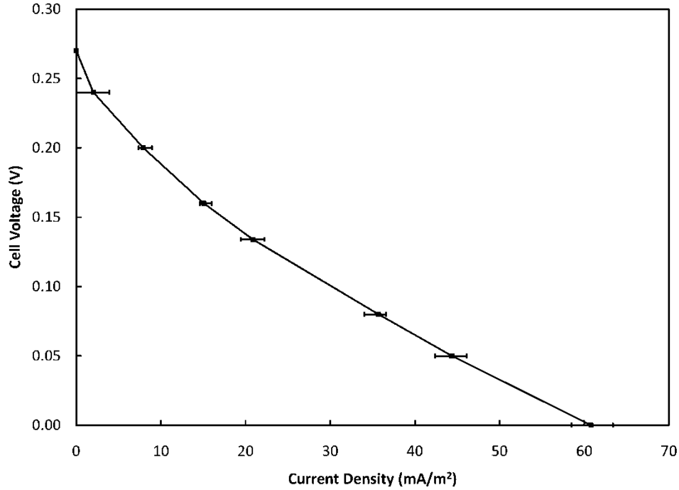
Figure 4.14. Polarization curve with bioanode (soluble mediator) with error bars. Data points are the average of three separate polarization curves on consecutive days and the bars are the range of the three measurements.
