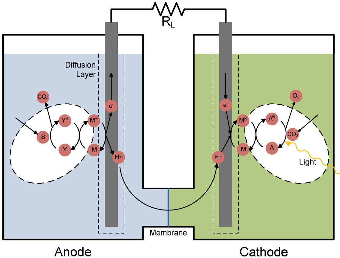
Figure 2.3. Diagram of a microbial fuel cell with a yeast bioanode and algae biocathode. A represents algae cells, Y represents yeast cells with superscripts 'R' representing the reduced state for those cells. S is the yeast substrate (glucose) and M is the mediator compound, either attached to the electrode or in solution depending on the experiment.
