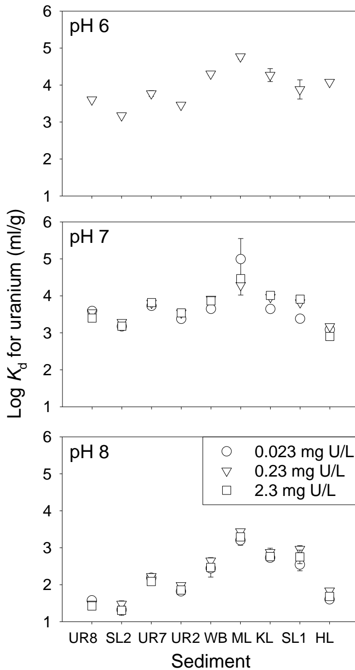
Fig. A4.1 Sediment partition coefficients (log K_d ; ml/g) for each sediment at three U concentrations (0.023, 0.23, and 2.3 mg/L) and at nominal pH levels of 6, 7 and 8. Data points represent mean values ( \pm SD, n = 2 ).
