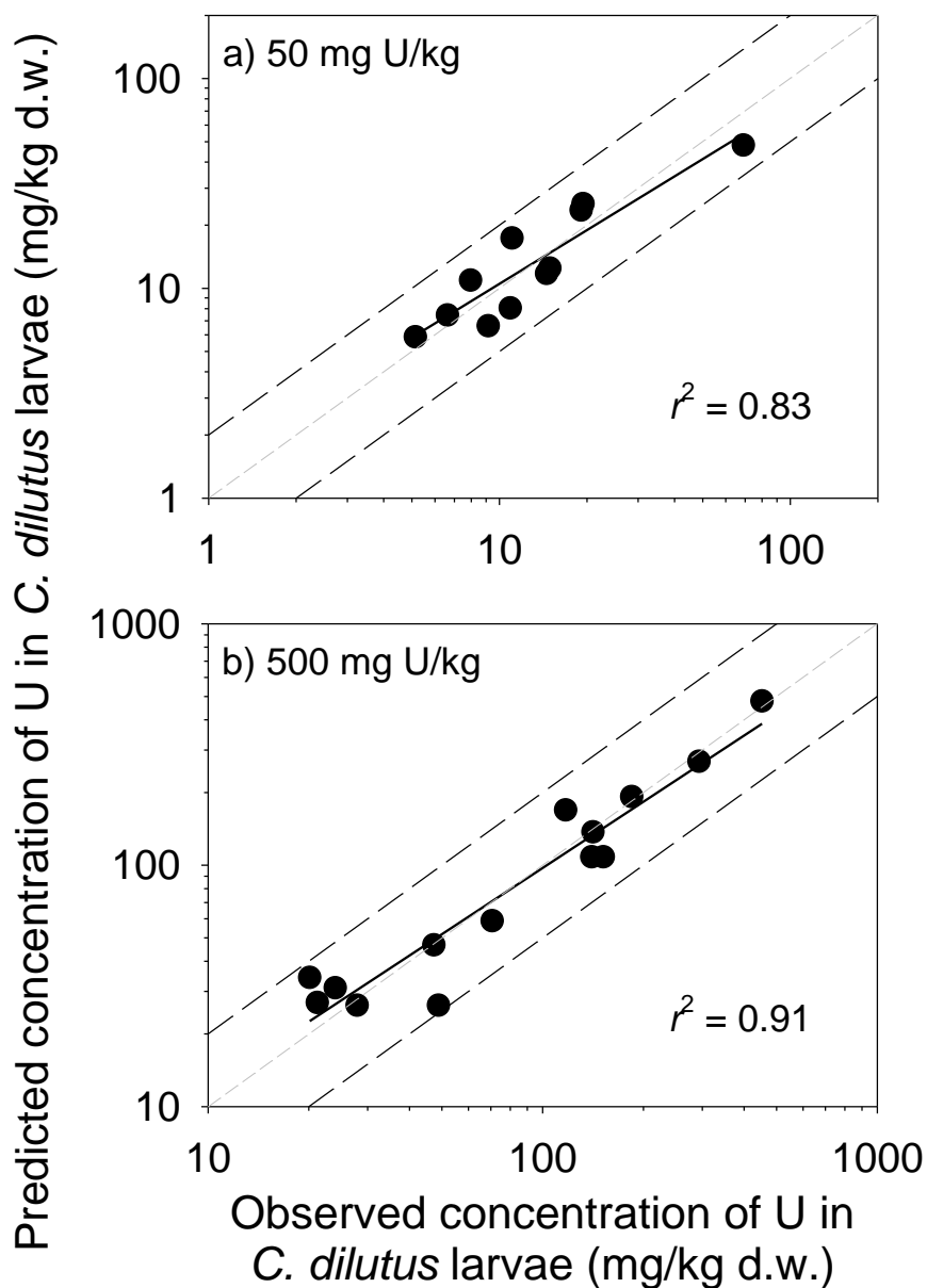
Fig. 3.3 Predicted versus observed bioaccumulation of U by C. dilutus larvae (mg/kg d.w.) in (a) 50 mg U/kg d.w. spiked field sediment based on bivariate regression analysis with fine fraction and Fe content as modifying factors (Eq. 3.1), and (b) 500 mg U/kg d.w. spiked field sediment based on univariate regression analysis with cation exchange capacity as the sole modifying factor (Eq. 3.2). The 1:1 line (dashed grey line) is bracketed by two-fold dashed lines (dashed black line) and presented with the linear regression (solid line).
