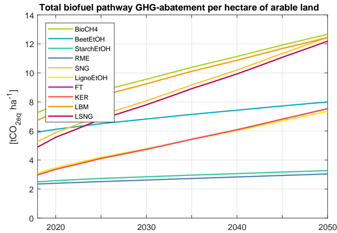
Figure 4: Development of greenhouse gas abatement per hectare [ \text{tCO}_{2eq} \text{ha}^{-1} ] for the biofuels included over the modelled time span, in the base scenario. Fischer-Tropsch-diesel shows exactly the same development as KER, and is therefore not visible in the graph.
