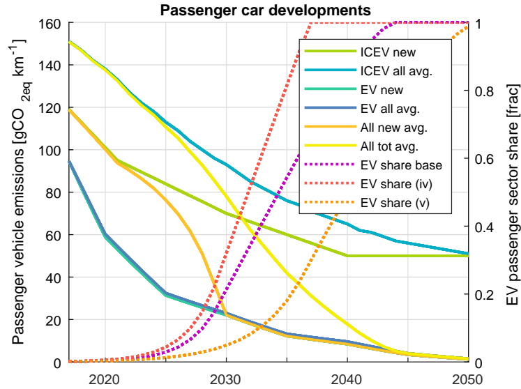
Figure 1: Passenger car sector developments. Average vehicle and fleet emissions are shown in solid lines [gCO 2eq km -1 , left axis]. The passenger sector market shares of EVs are shown in dotted lines [frac, right axis], for the base case as well as for scenarios (iv) where EVs have a 50% higher usage rate and (v) where the EV growth rate is at 30% a -1 . From 2030 onwards, EVs make up all new passenger cars. The fleet emissions including EVs compared to with only ICEVs diverge at higher shares of EVs, combined with a cleaner power system and the fact that also older EVs improve their driving emissions according to the changing power system.
