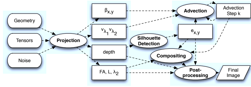
Fig. 1 Flowchart indicating the four major steps of the algorithm: projection , which transforms the data set in an image-space representation and produces the initial noise texture on the geometry; silhouette detection , required for the advection step and the final rendering; advection , which produces the two eigenvector textures; compositing , which combines intermediate textures; and the postprocessing , which adds additional shading and improves the perceptual quality of the final visualization. Between consecutive steps, the data is transferred using textures.
