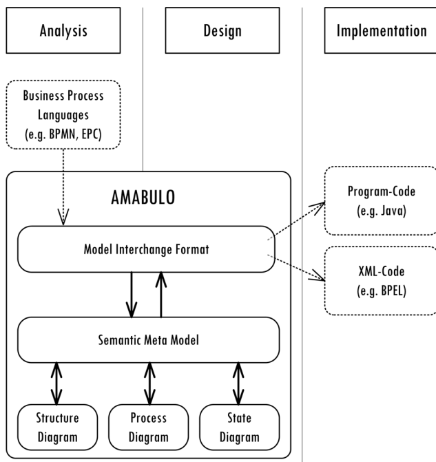
Figure 1. Overview over Model Architecture
