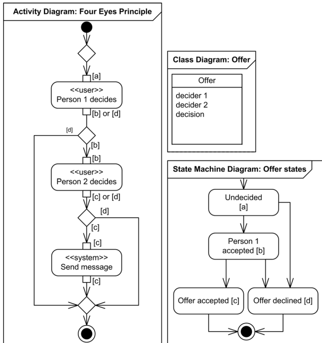
Figure 4. Four Eyes Principle as Example Model
