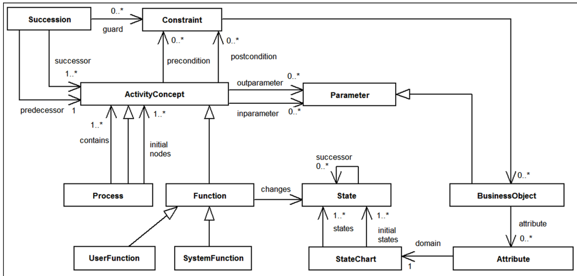
Figure 2. Meta Model
