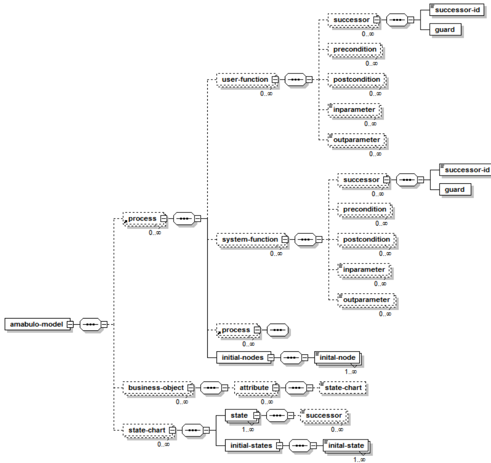
Figure 5. AMABULO Interchange Format
