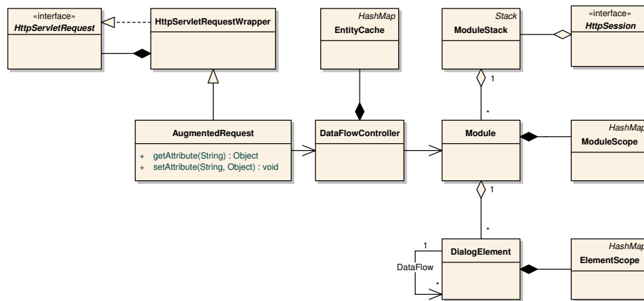
Fig. 6. Data flow control logic of the Dialog Control Framework
