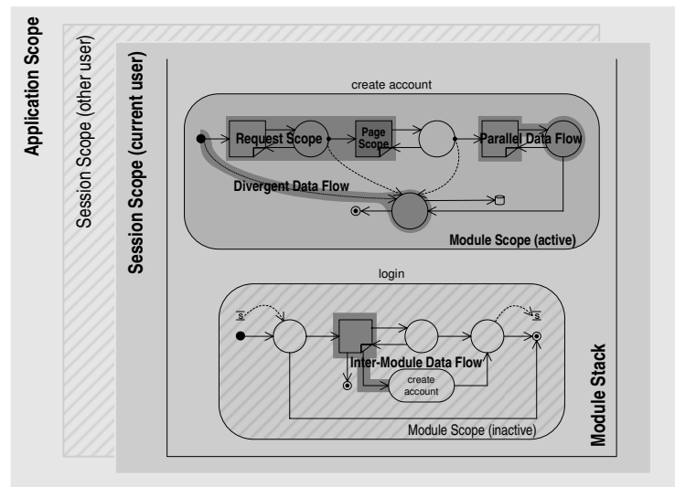
Fig. 4. Scopes and data flows supported by the Dialog Flow Notation and Dialog Control Framework
