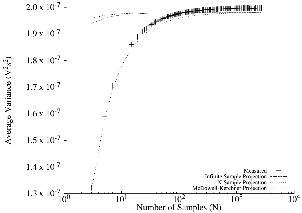
Figure 4.10: White Noise Sample Sequence Variance, \Delta T = 1\text{s} , T = 0.02\text{s}
