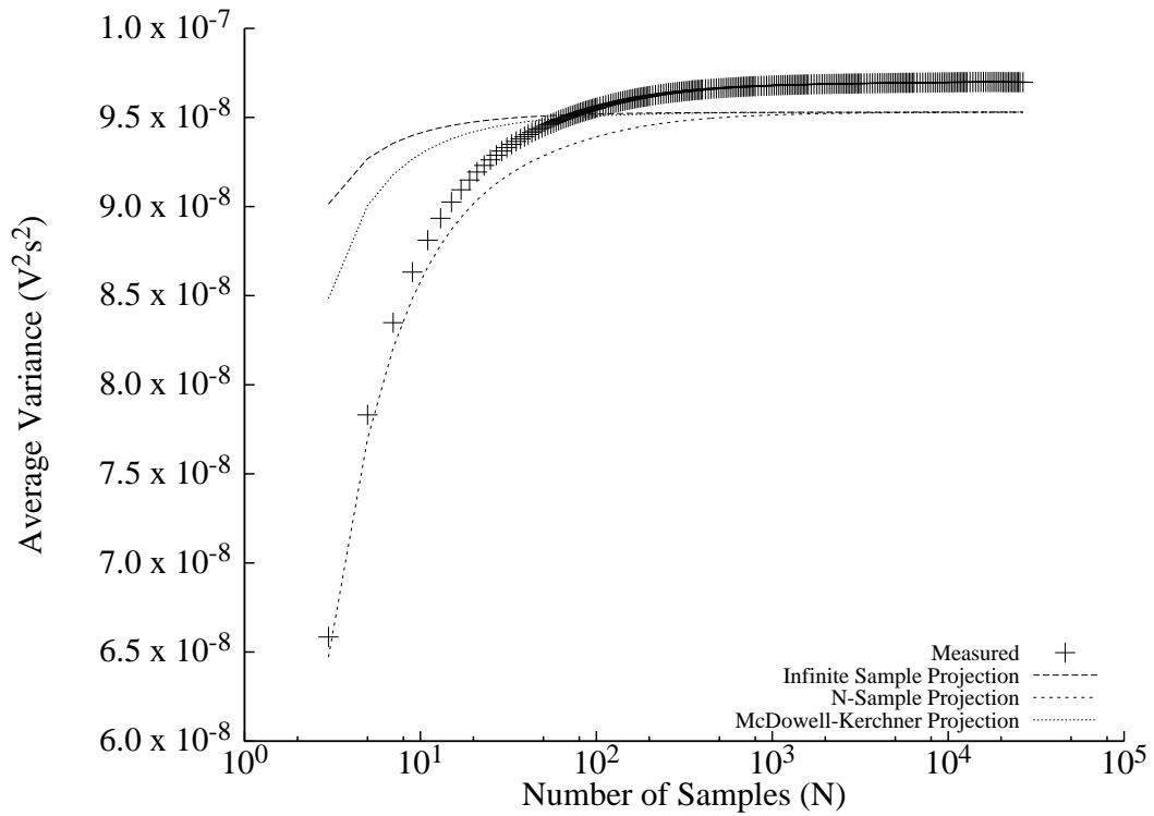
Figure 4.11: White Noise Sample Sequence Variance, \Delta T = 0.1\text{s} , T = 0.01\text{s}
