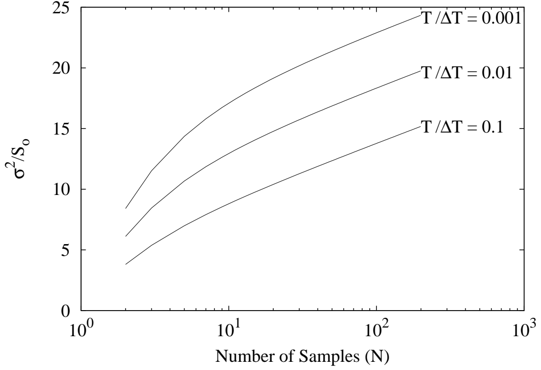
Figure 3.3: Normalized variance of N samples at different 1/\zeta for \alpha = 1
