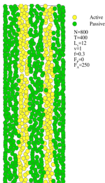
Figure 18: lane formation.
