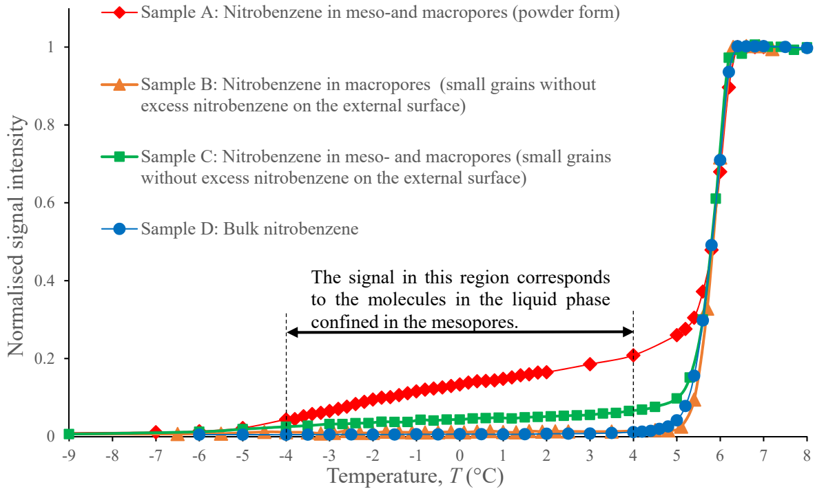
Figure 3. Melting curves of nitrobenzene in different samples. (A) Nitrobenzene in meso- and macropores (powder form). (B) Nitrobenzene in macropores (small grains without excess nitrobenzene on the external surface). (C) Nitrobenzene in meso- and macropores (small grains without excess nitrobenzene on the external surface). (D) Bulk nitrobenzene
