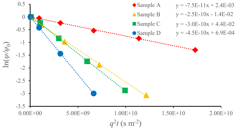
Figure 5. Spin-echo attenuation plots for t = 40 ms. (A) Solely mesopores. (B) Solely macropores. (C) Both meso- and macropores. (D) Bulk nitrobenzene
