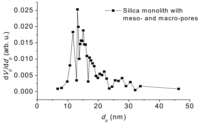
Figure 4. Pore size distribution of the hierarchically porous silica monolith with meso- and macropores, obtained from NMR cryoporometry. The solid line serves as a guide to the eye.
