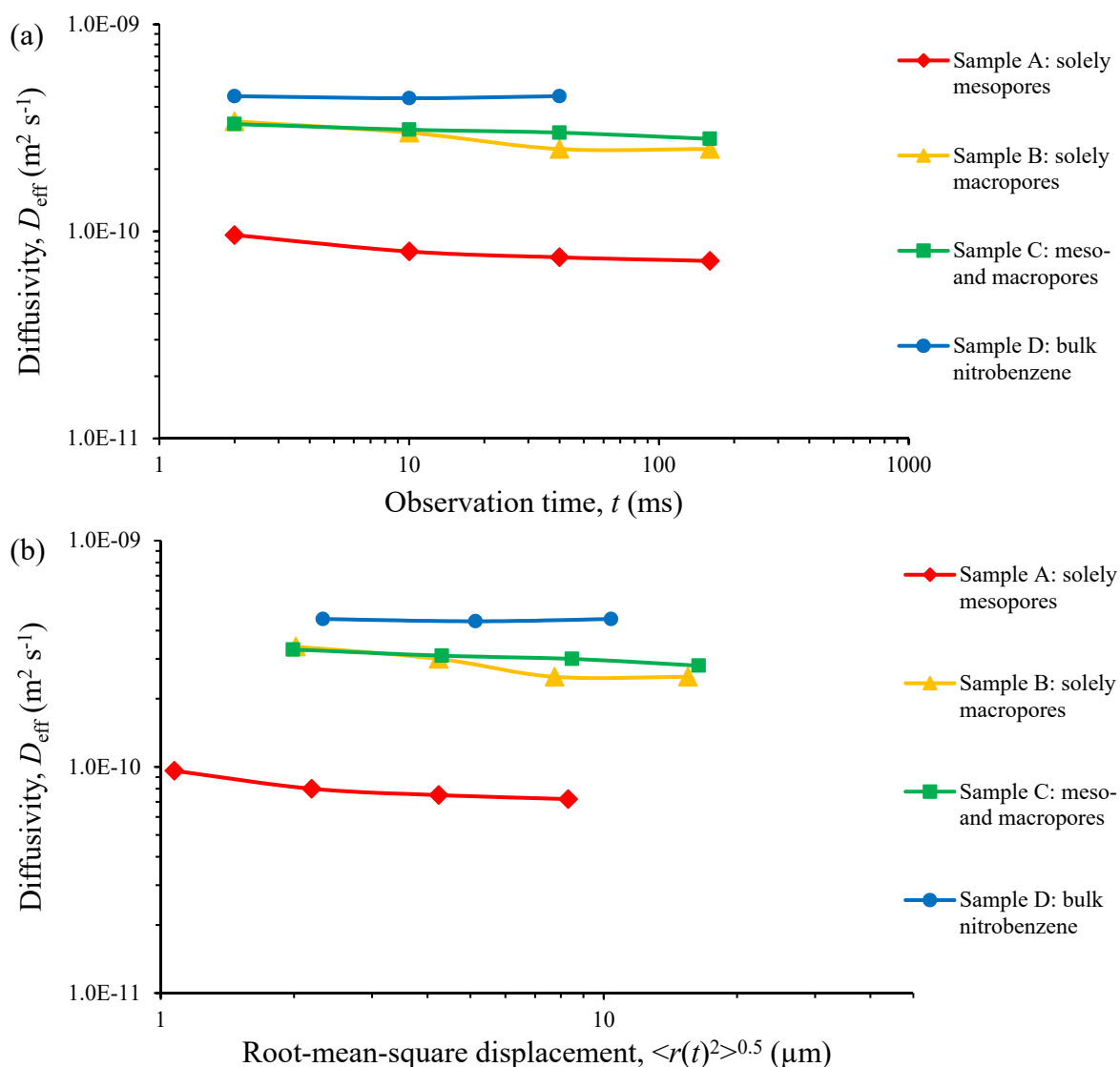
Figure 6. Diffusivities for nitrobenzene as a function of observation time (a) and root-mean-square displacement (b)
