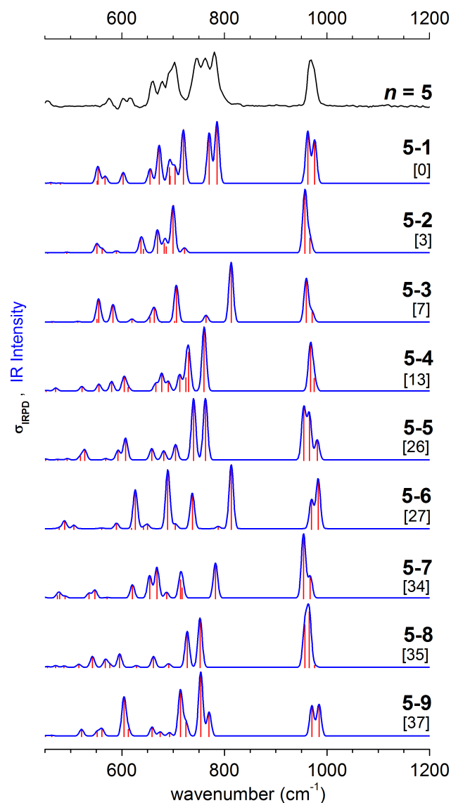
FIG. 4. Smoothed experimental IRPD spectrum (black) of D_2 -tagged (TiO_2)_n^- ( n = 5 ) and simulated linear IR absorption traces (blue), stick spectra (red), and relative energies (kJ/mol) of the predicted lowest-lying isomers at the BP86/6-311+G* level of theory.
