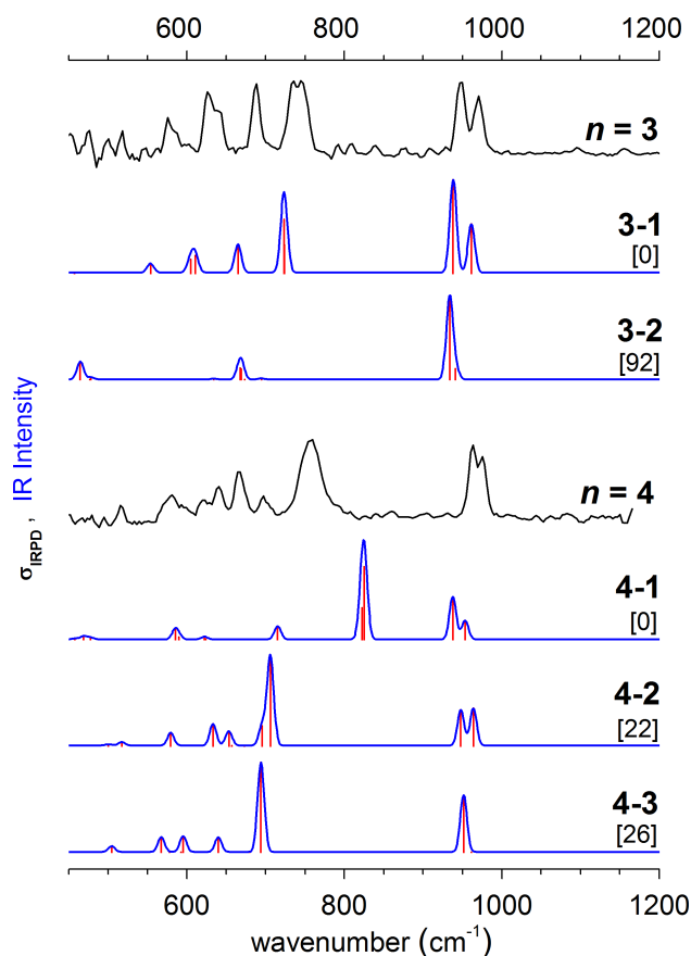
FIG. 3. Smoothed experimental IRPD spectra (black) of D_2 -tagged (TiO_2)_n^- ( n = 3, 4 ) and simulated linear IR absorption traces (blue), stick spectra (red), and relative energies (kJ/mol) of the predicted lowest-lying isomers at the BP86/6-311+G* level of theory.
