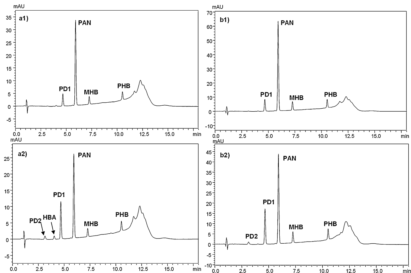
Fig. 1. LC-UV (method A; \lambda_a = 254 nm) chromatograms of PAN in 0.01 M NaOH solution at room temperature (a1) t = 5 h; (a2) t = 8 h) and in 0.1 M HCl solution (b1) t = 25 °C, t = 24 h; (b2) t = 45 °C, t = 6 h).
