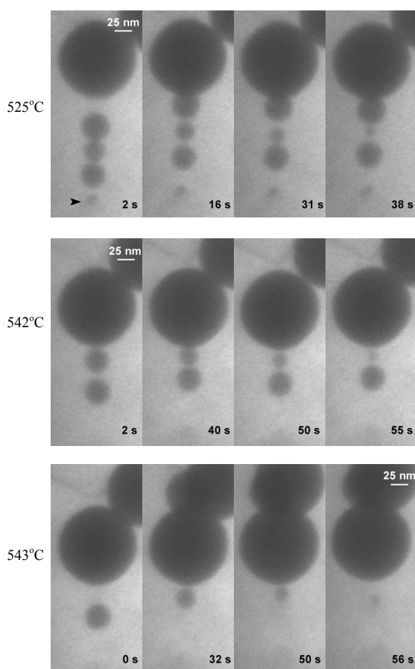
Fig.1. In-situ TEM observations of dissolution of the inclusions. The arrow shows termination of the dislocation at the free surface of the foil.
