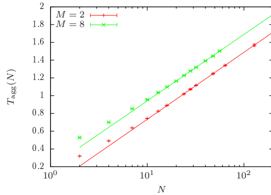
Figure 3.11.: Scaling of the aggregation transition temperature for fixed M and increasing N . The rescaled density is M/L^3 = 0.1 , such that L' = L/N is fixed for each curve.
