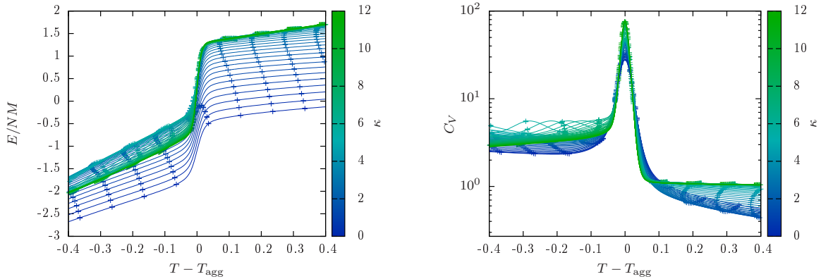
Figure 4.3.: Effect of stiffness on the canonical estimates of the average energy (left) and specific heat (right) for 8 semiflexible polymers of length N = 13 ( \rho_m = 10^{-3} ). The temperature is shifted around the aggregation temperature T_{\text{agg}} and the graph color encodes the bending stiffness \kappa in the interval [0, 12] with \Delta\kappa = 0.2 .
