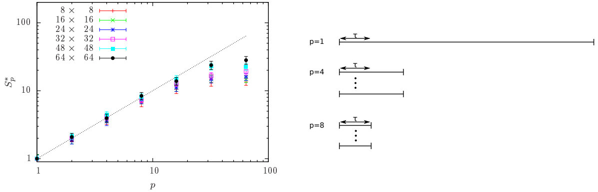
Figure 5.5.: (left) Statistical speedup factor for the 8-state Potts model with increasing system size. (right) Scheme of \bar{N}_{\text{iter}}/\text{core} compared to the integrated autocorrelation time \tau demonstrating the natural limit of parallelization [120].
