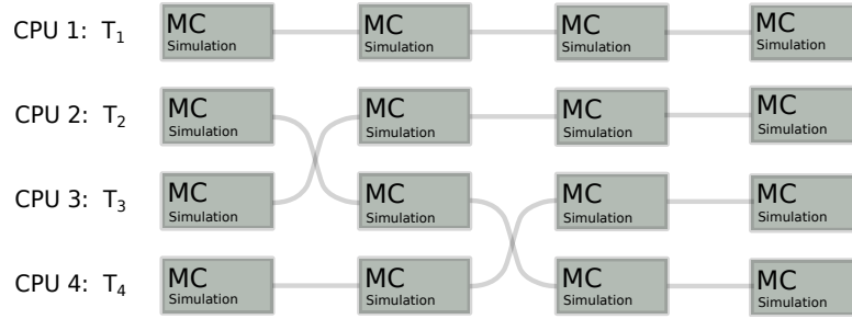
Figure 5.1.: Scheme of parallel tempering taken from Ref. [124]. The system is simulated for a set of temperatures in parallel with the possibility that two Markov chains may exchange configurations according to Eq. (5.17).
