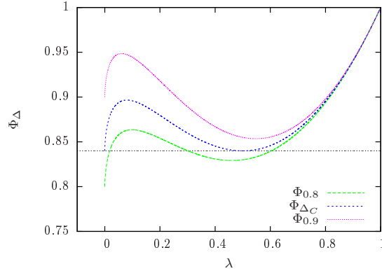
Figure 2.7.: The reduced free-energy function \Phi_{\Delta}(\lambda) in three dimensions for several values of \Delta around the transition “density” \Delta_c . The minimum is either at \lambda = 0 , namely \Phi_{\Delta}(0) = \Delta for \Delta < \Delta_c or at a non-trivial value of \lambda > \lambda_c .
