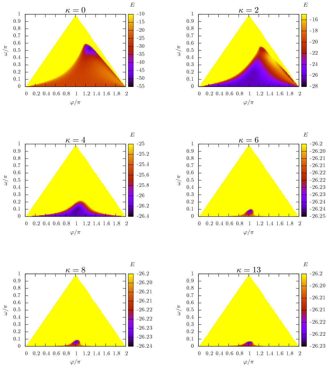
Figure 4.9.: Total energy E_{LJ}(\varphi, \omega) + \kappa 2(N - 2)(1 - \cos\theta(\varphi, \omega)) from numerical variation of \varphi and \omega for the 2 \times 13 twisted polymers parameterization for several \kappa .
