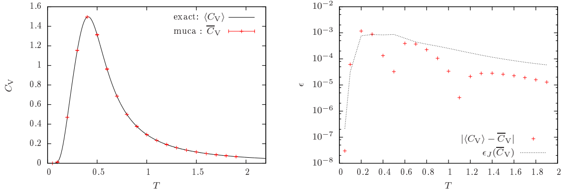
Figure 2.3.: Same as Fig. 2.2 for the specific heat estimator \overline{C}_V and exact expectation value \langle C_V \rangle .
