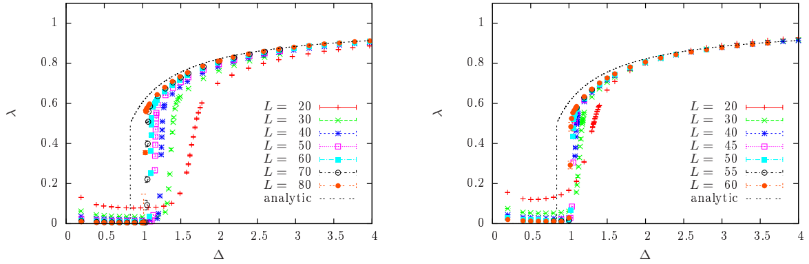
Figure 2.11.: Condensation of a lattice gas in three dimensions at two temperatures around the roughening temperature T_R : T = 0.5 < T_R (left) and T = 0.8 > T_R (right). The numerical data from multicanonical simulations show strong finite-size corrections compared to the analytical solution (dashed line).
