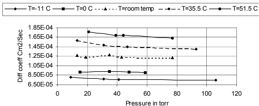
Figure 1. Argon diffusivities at different temperatures as a function of pressure
