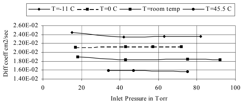
Figure 2. Helium diffusivities at different temperatures as a function of pressure
