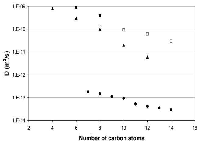
Figure 2. Comparison of experimental results at 423K. ■ QENS new data; □ QENS [1]; ▲ PFG-NMR ; ● ZLC.
