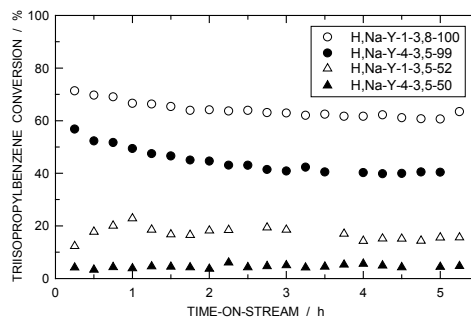
Figure 2: Catalytic conversion of 1,3,5-triisopropylbenzene over zeolite H,Na-Y.
