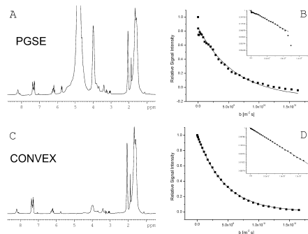
Fig. 2. Representative spectra and attenuation plots from conventional PGSE (A, B) and CONVEX (C, D).
