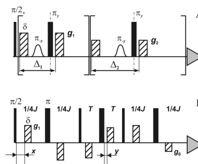
Fig. 1. Pulse sequences of: (A) CONVEX; (B) DQDiff.
