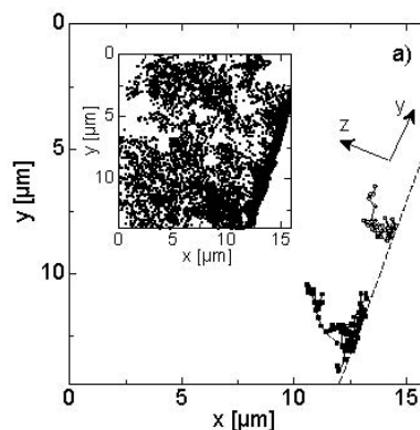
Figure 1: Two single molecule trajectories. Molecules diffuse along the surface step. Inset: Trajectory points of all molecules. Surface step in the lower right corner.
