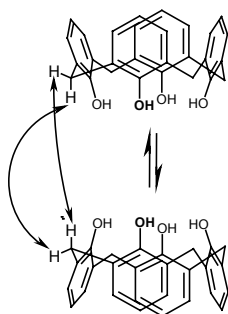
Fig. 2: Cone - " inverted cone " transition
