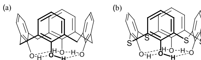
Fig. 1: Calix[4]arene (a) and thiacalix[4]arene (b) with the circular hydrogen bond array on the lower rim
