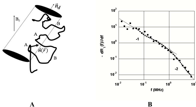
Fig.1: A: Intermittent Brownian dynamics over a strand. A and B stand for the Adsorption step and the Relocation (Bridge statistics). B: Frequency dependence of the spin-lattice relaxation rate in diluted suspension of imogolite. Full squares: experimental results. Dotted line: Brownian dynamics numerical simulation.
