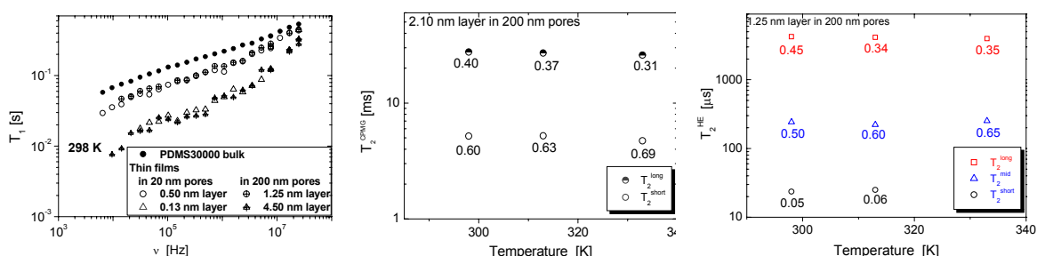
Fig 1. ^1\text{H} relaxation times for PDMS ( M_w=33300 g/mol) in Anopore membranes. (a) left : T_1 dispersion of PDMS of different layer thicknesses in two different pore sizes. (b) center : T_2 values determined by CPMG for a 2.10 nm layer in 200 nm pores. (c) right : T_2 values determined by Hahn echo for a 1.25 nm layer in 200 nm pores. Numbers below the symbols denote the weight fraction of the corresponding component.
