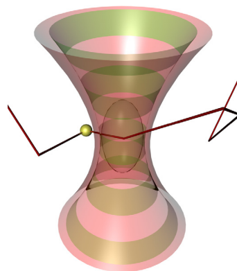
Fig. 1: PhoCS working principle – a colloidal particle enters the focal domain, is heated and the resulting change in solvent index of refraction is detected.
